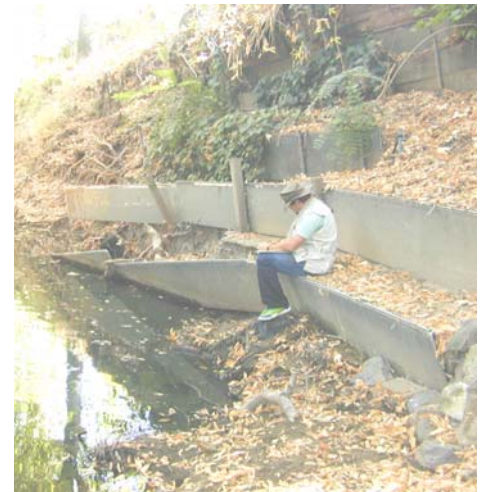
Crib Wall in Alhambra Creek, CA
